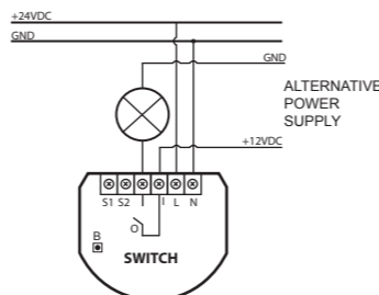
Fig.1 Wiring diagrams for Fibaro Switch.
