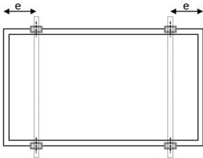
Fig. A2: Clipping position on long frames
