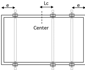
Fig. A1: Clipping position on long frames
